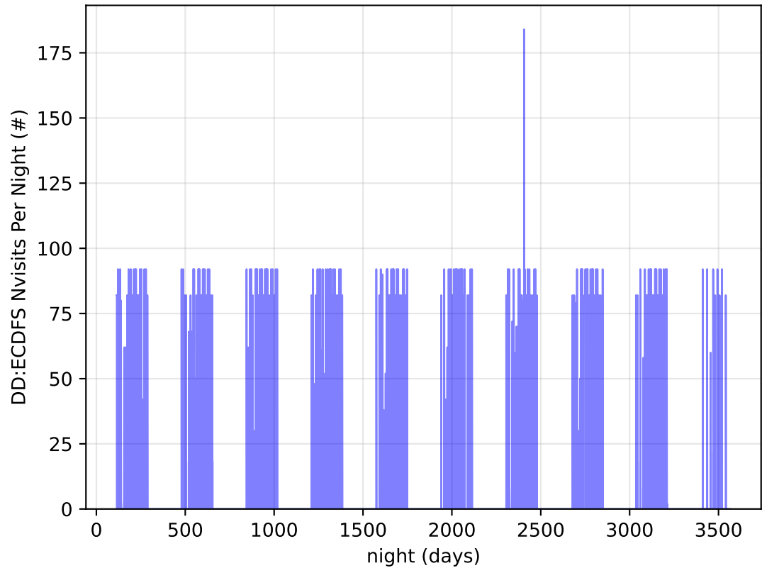
ddf_acor_sf25_lsf40_lsr50_v3.4_10yrs all bands: DD:ECDFS Nvisits Per Night
