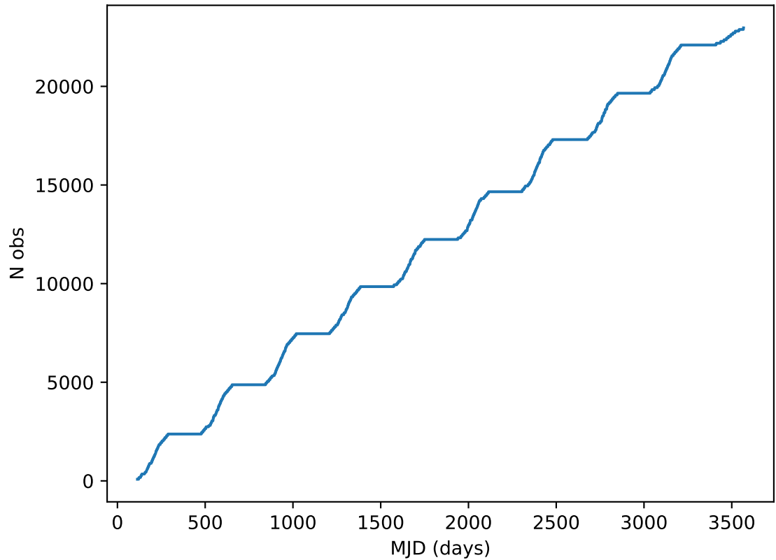
ddf_acor_sf25_lsf40_lsr50_v3.4_10yrs all bands: DD:ECDFS Cumulative NVisits
