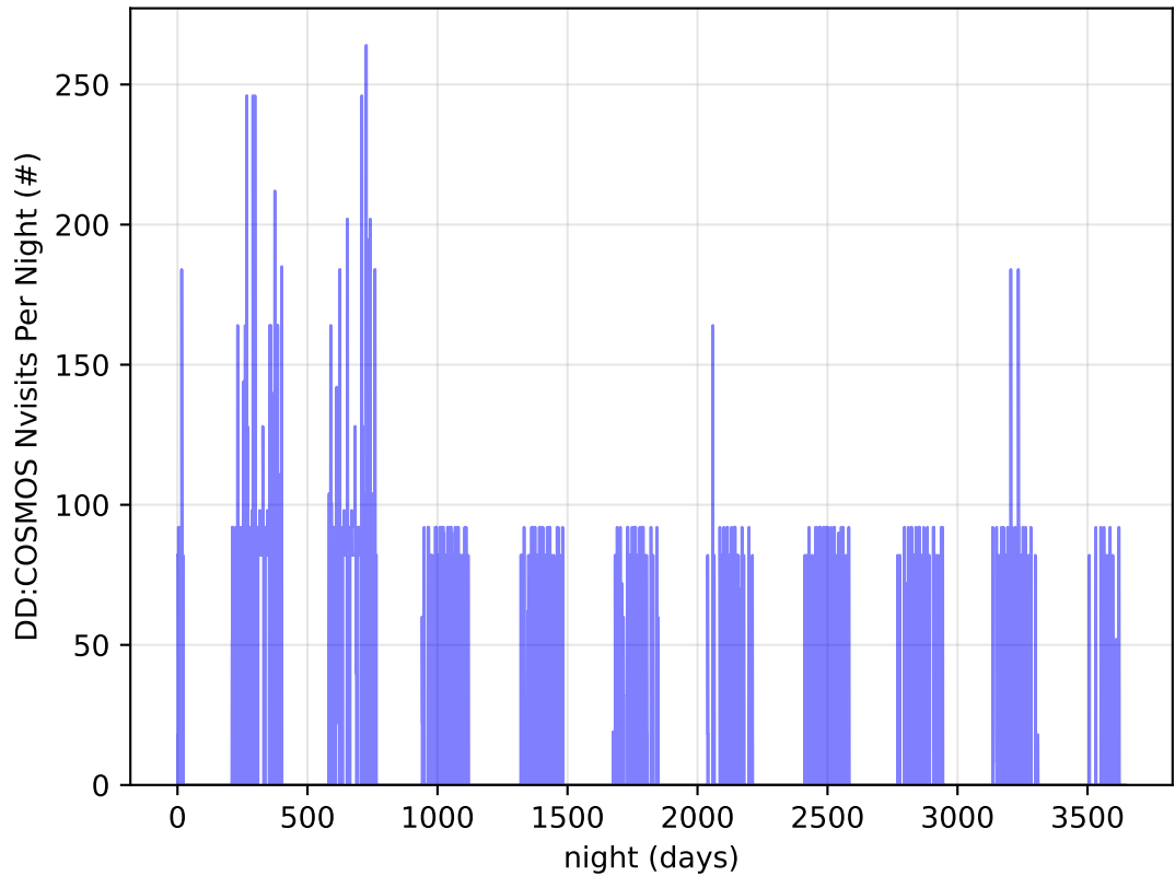
ddf_acor_sf25_lsf40_lsr50_v3.4_10yrs all bands: DD:COSMOS Nvisits Per Night
