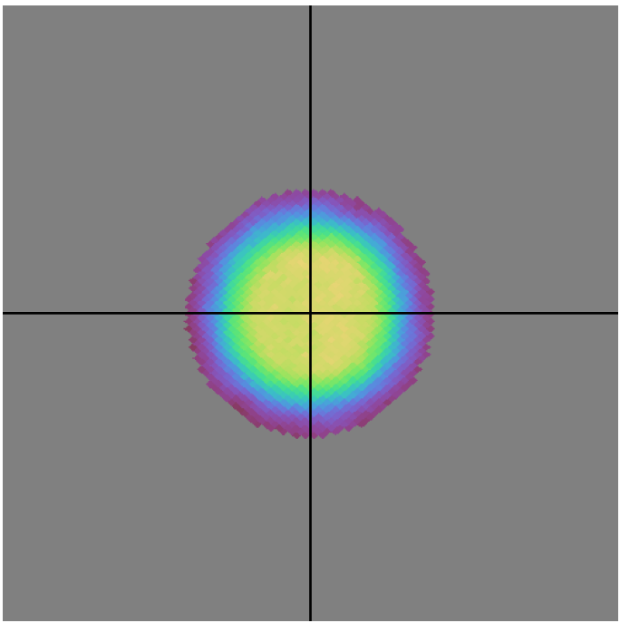
ddf_acor_sf25_lsf40_lsr50_v3.4_10yrs all bands: DD:COSMOS N Unique Nights
