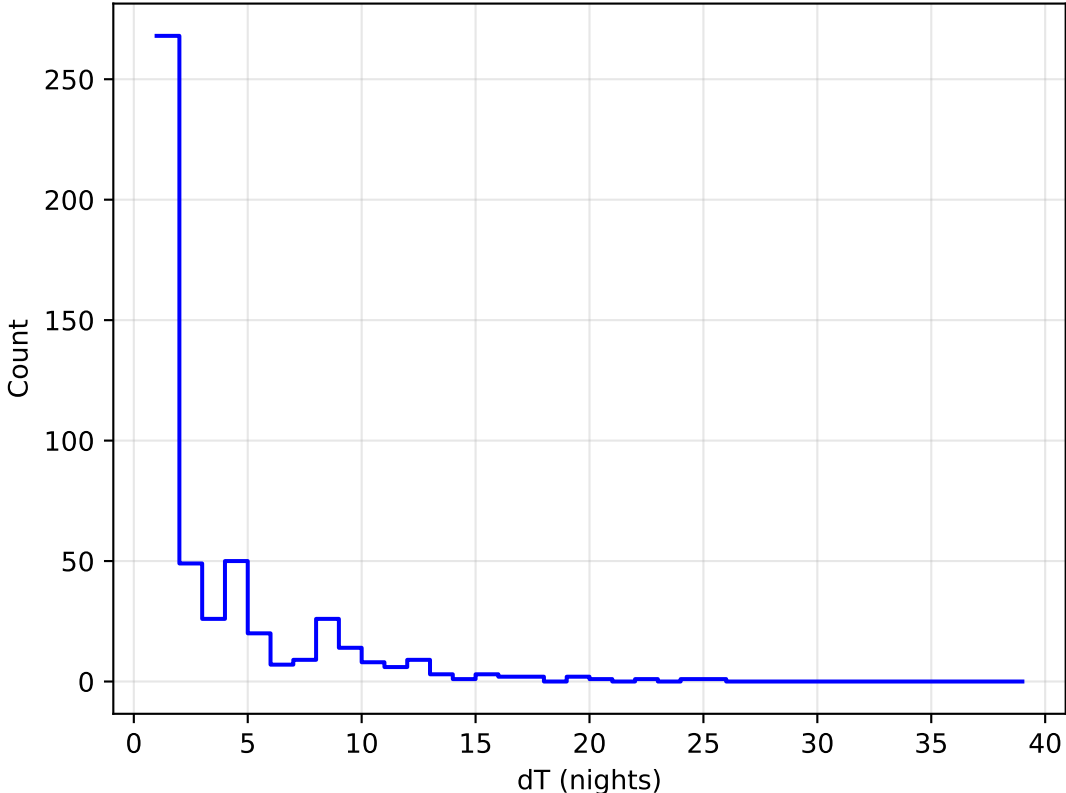
ddf_acor_sf25_Isf40_Isr50_v3.4_10yrs all bands: DD:COSMOS Delta Nights Histogram
