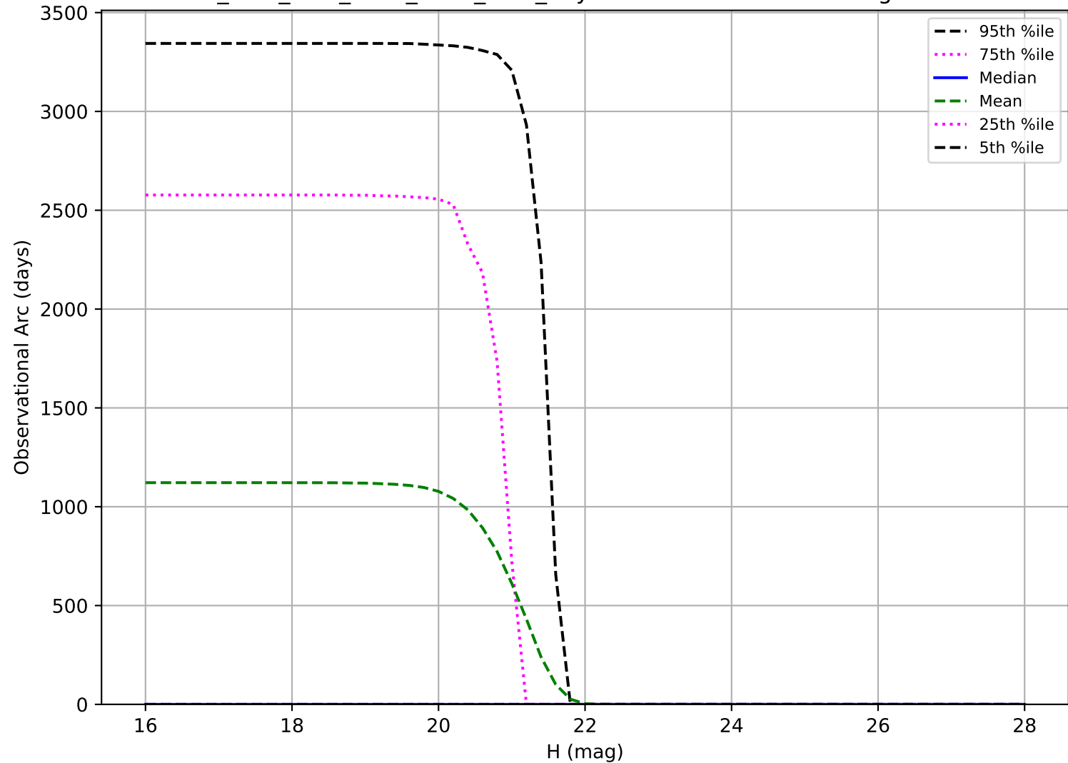
ddf_acor_sf25_lsf40_lsr20_v3.4_10yrs: Observational Arc Length Vatira
