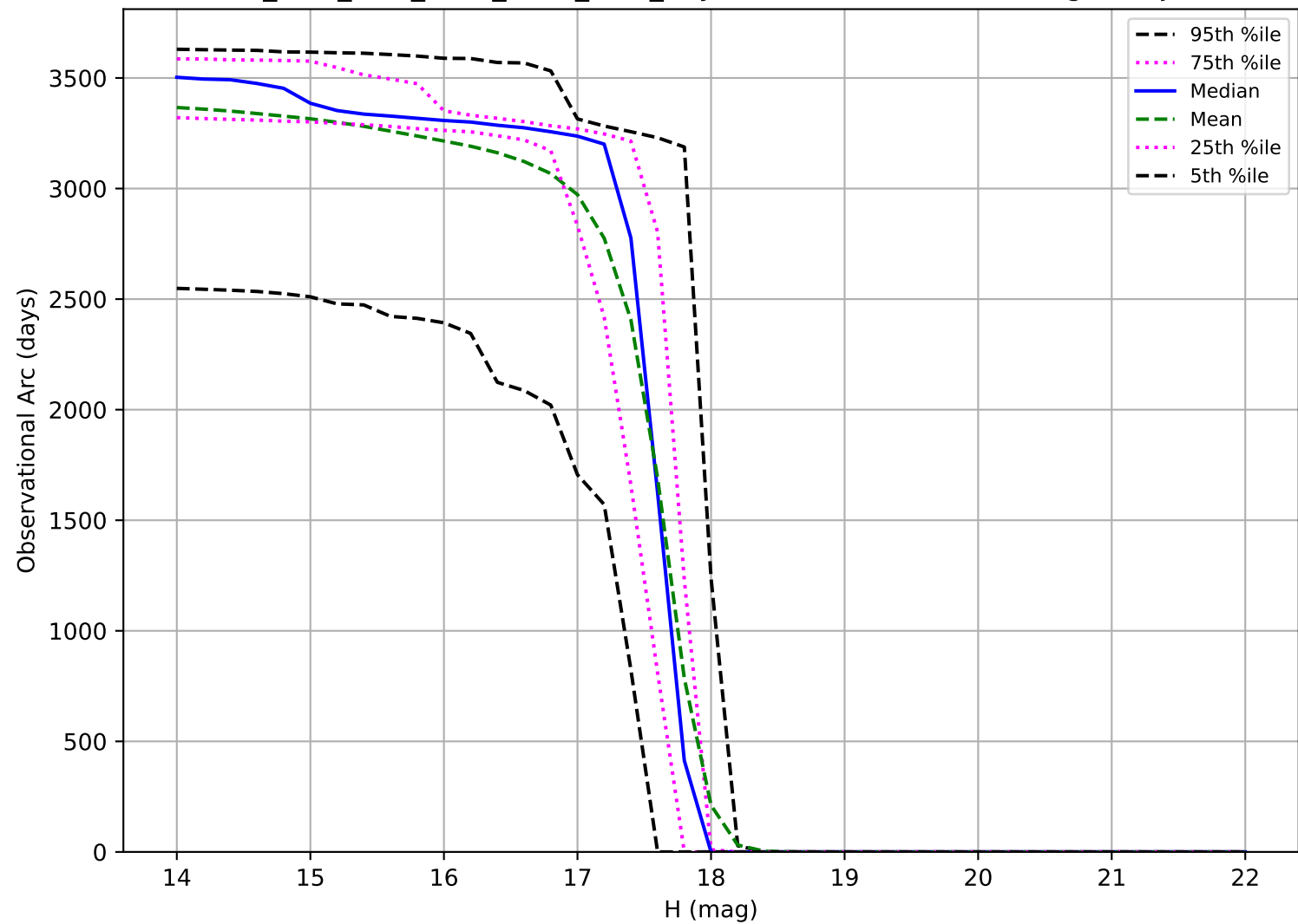
ddf_acor_sf25_lsf40_lsr20_v3.4_10yrs: Observational Arc Length Trojan
