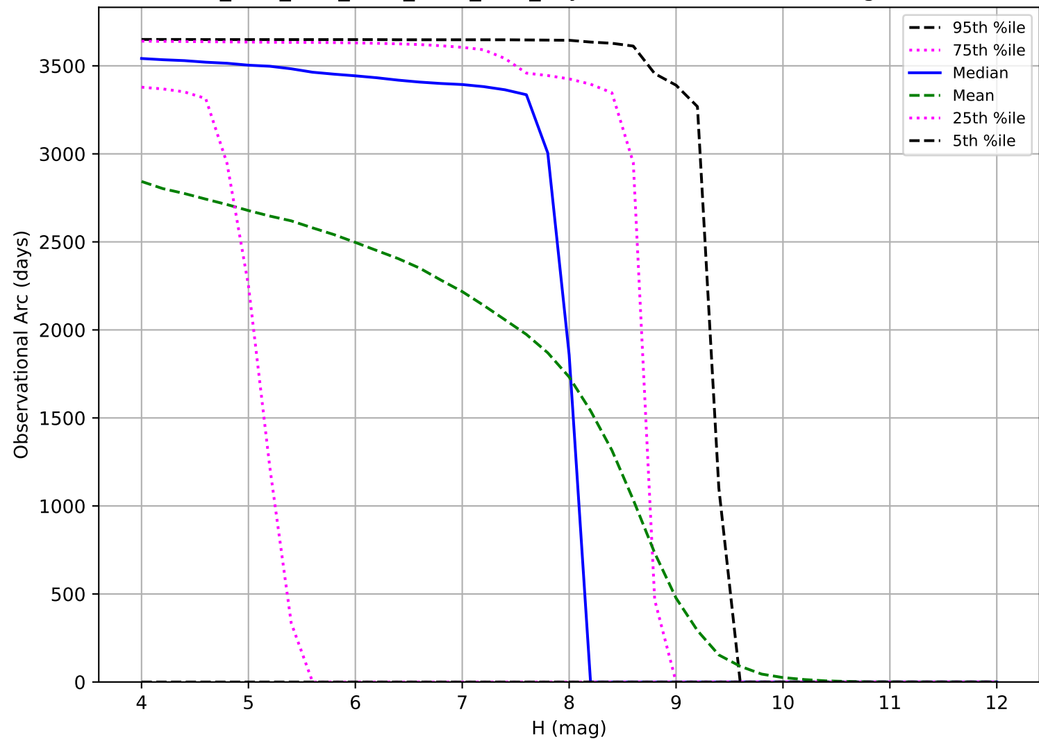
ddf_acor_sf25_Isf40_Isr20_v3.4_10yrs: Observational Arc Length TNO
