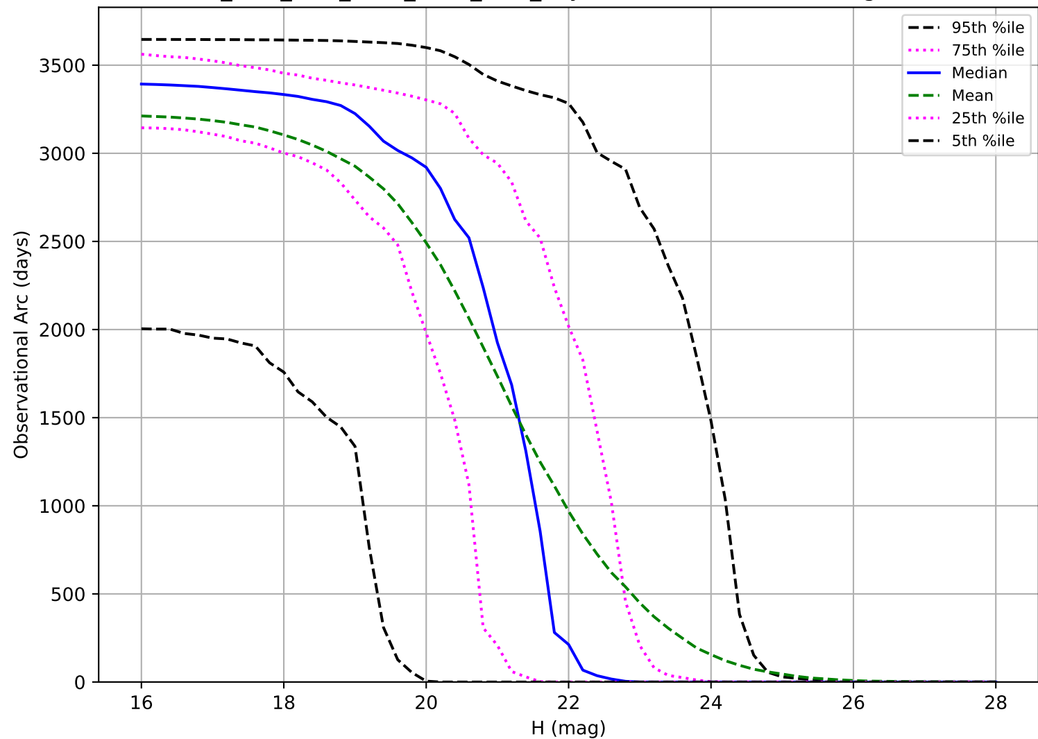
ddf_acor_sf25_lsf40_lsr20_v3.4_10yrs: Observational Arc Length PHA
