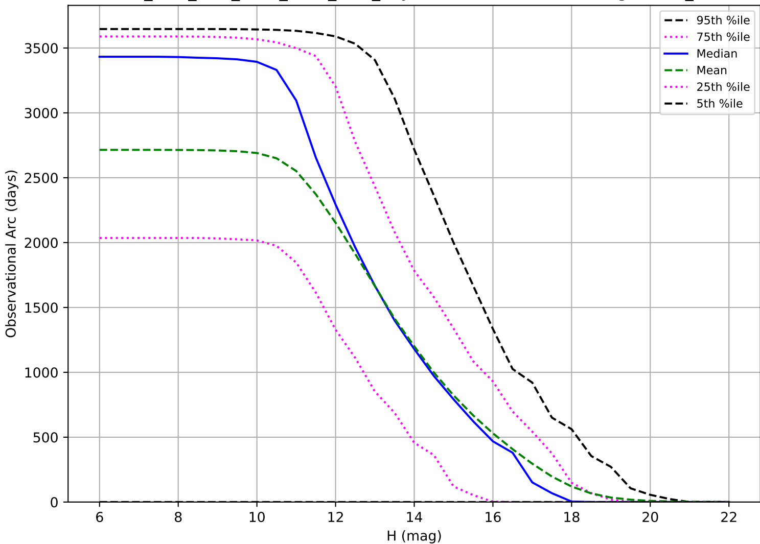
ddf_acor_sf25_lsf40_lsr20_v3.4_10yrs: Observational Arc Length OCC_r5
