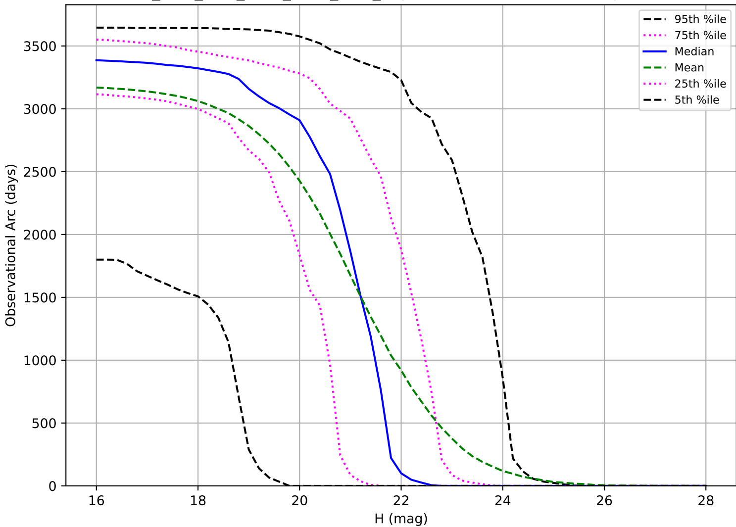
ddf_acor_sf25_Isf40_Isr20_v3.4_10yrs: Observational Arc Length NEO
