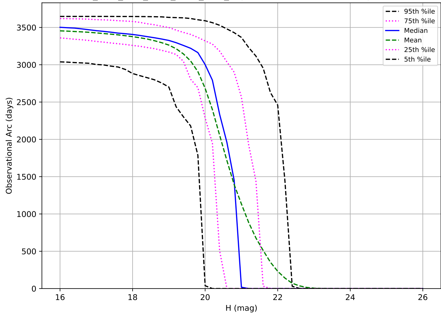
ddf_acor_sf25_lsf40_lsr20_v3.4_10yrs: Observational Arc Length MBA
