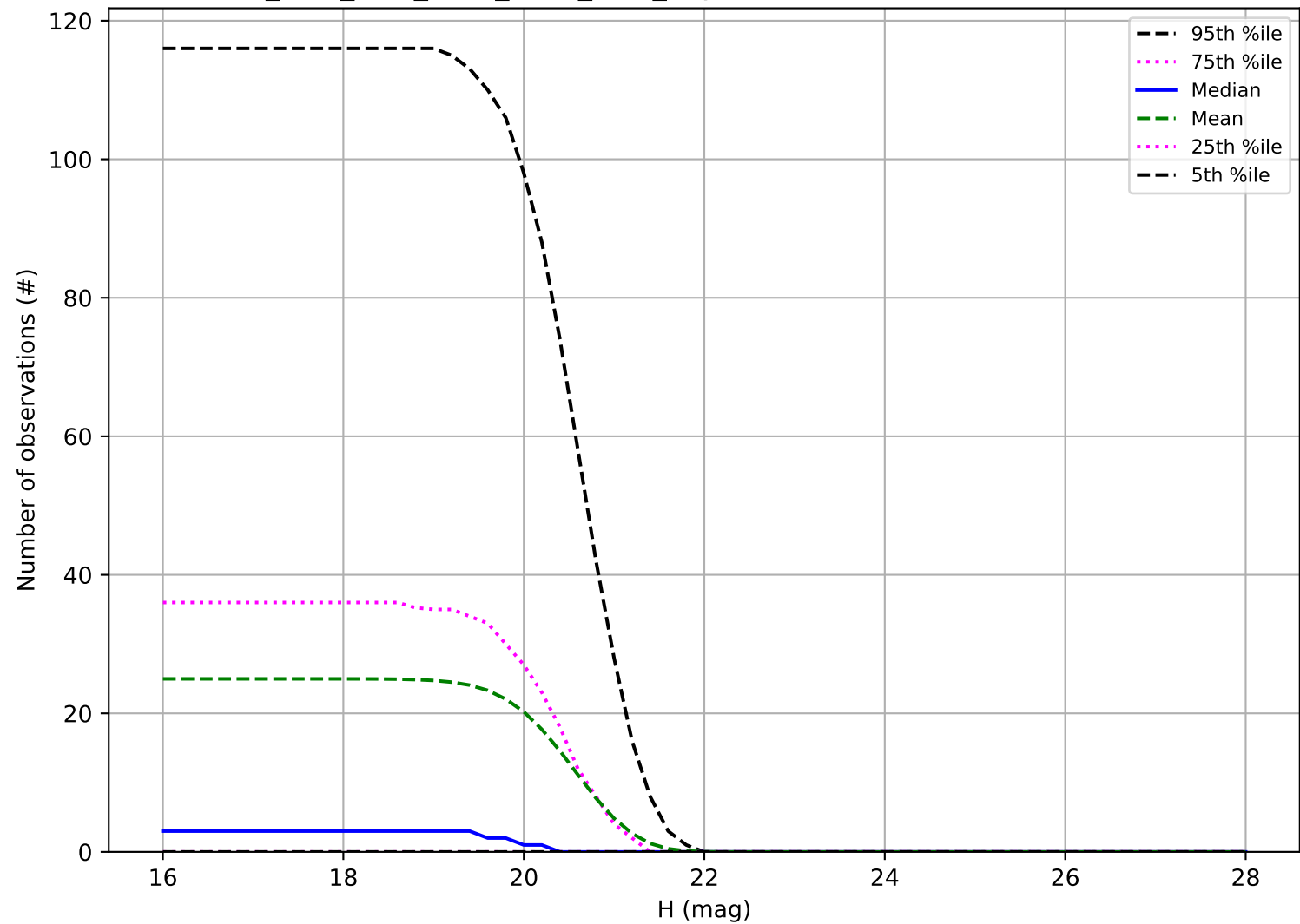
ddf_acor_sf25_lsf40_lsr20_v3.4_10yrs: Number of observations Vatira
