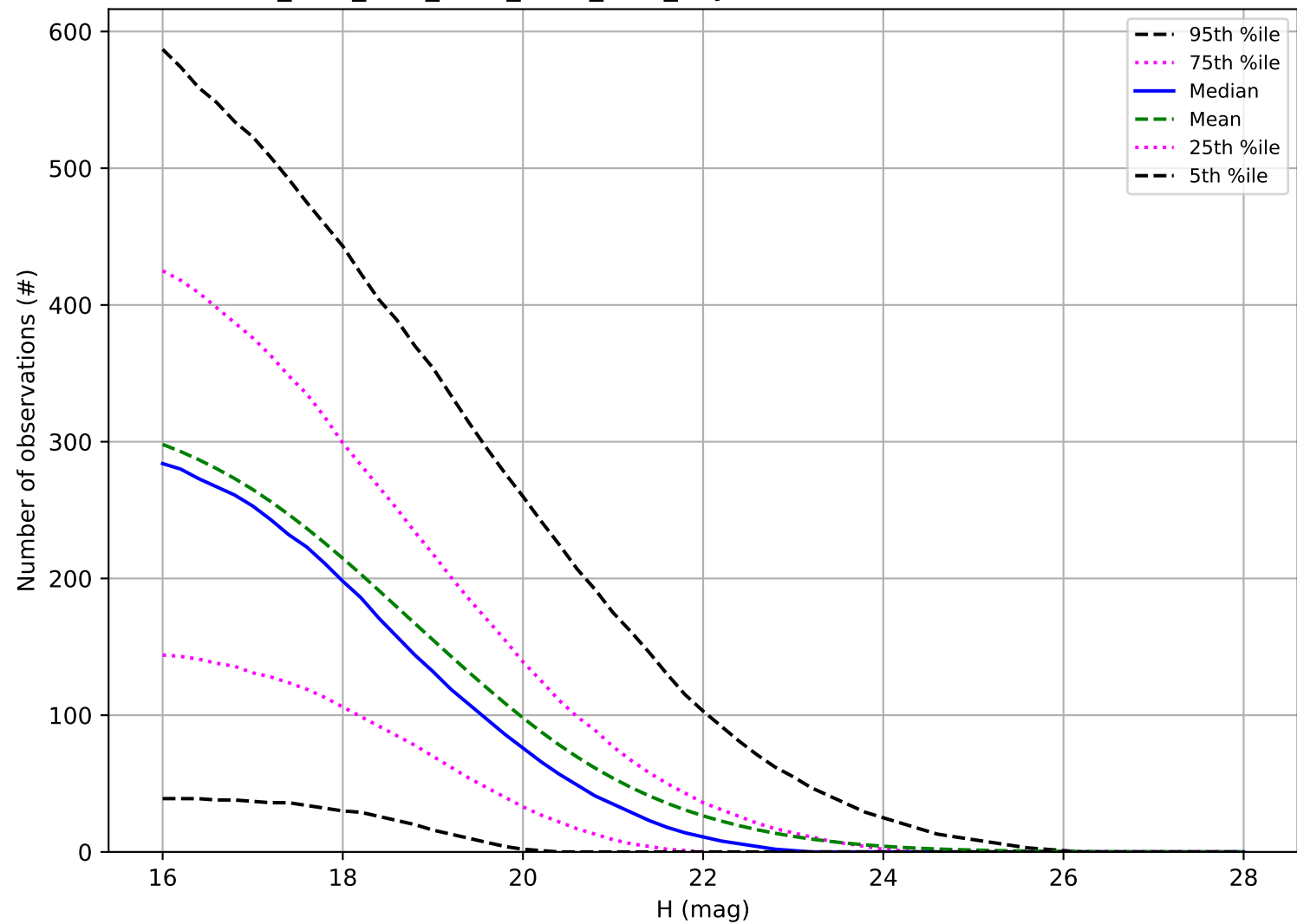
ddf_acor_sf25_lsf40_lsr20_v3.4_10yrs: Number of observations PHA
