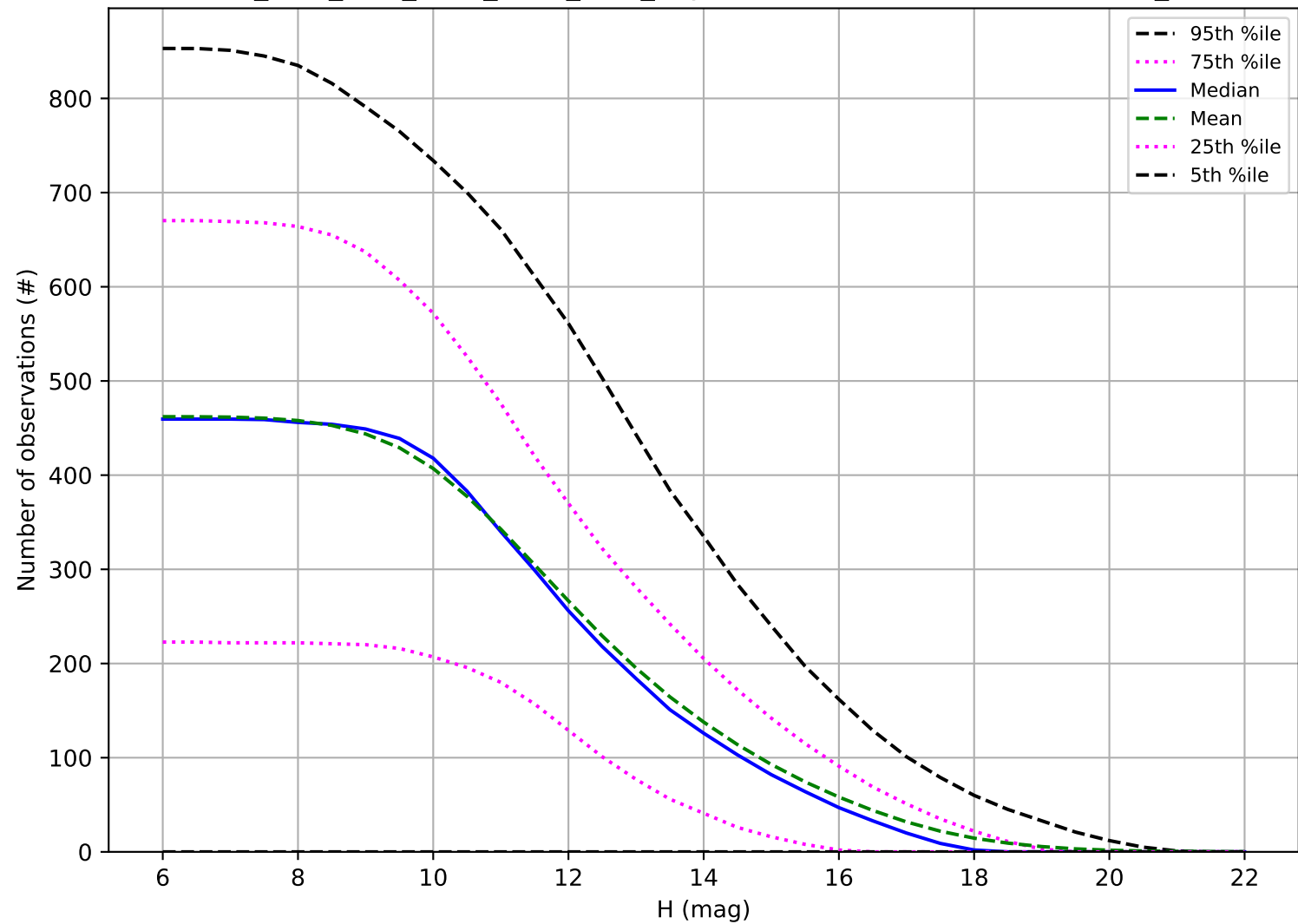
ddf_acor_sf25_lsf40_lsr20_v3.4_10yrs: Number of observations OCC_r5
