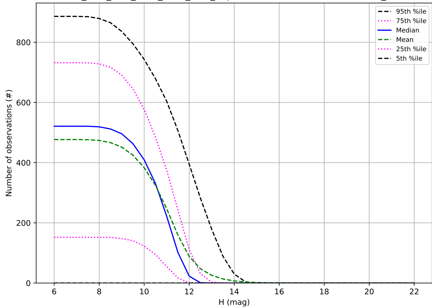
ddf_acor_sf25_lsf40_lsr20_v3.4_10yrs: Number of observations OCC_r20
