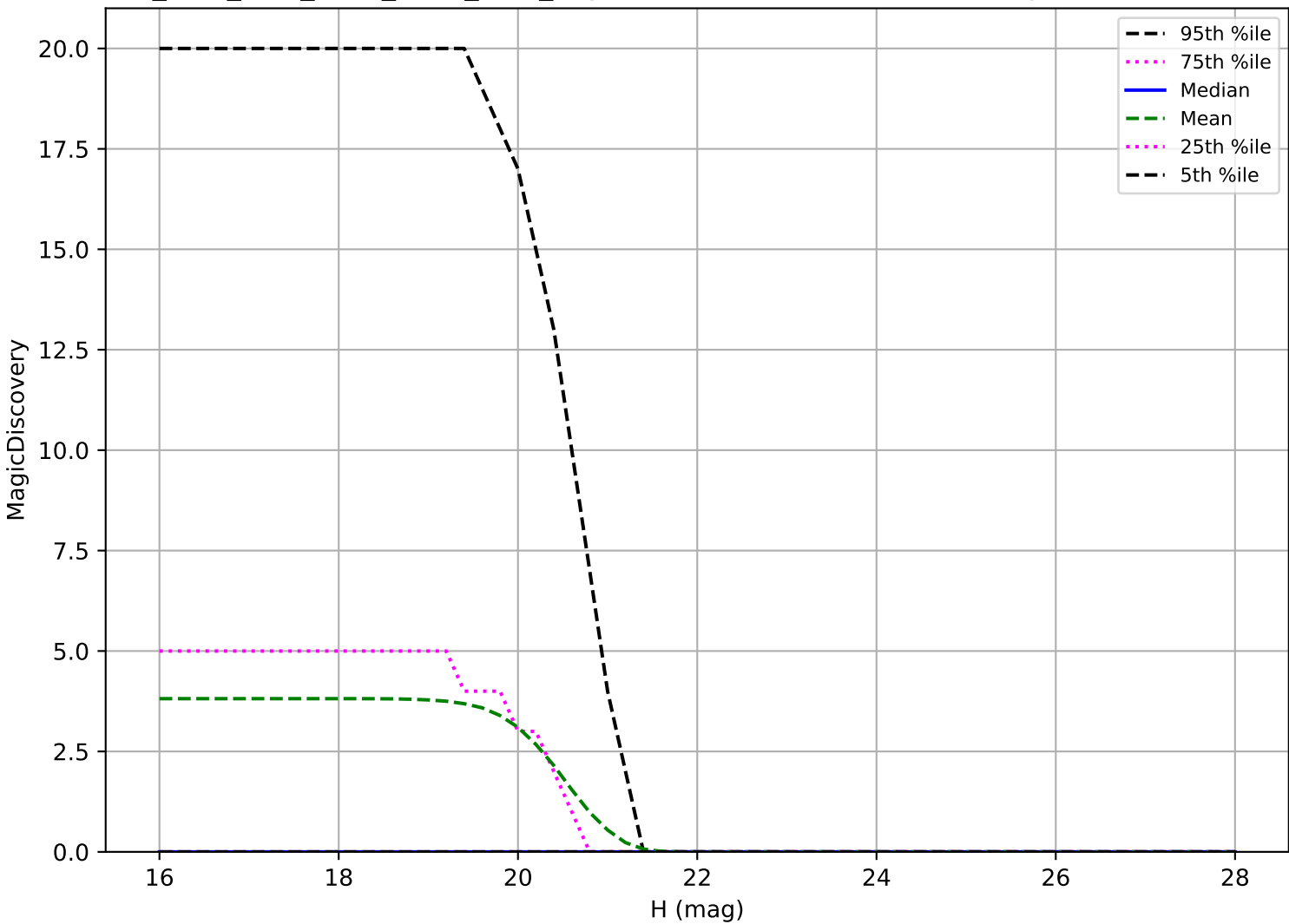
ddf_acor_sf25_lsf40_lsr20_v3.4_10yrs: Vatira 6 detections in 60 nights detection loss
