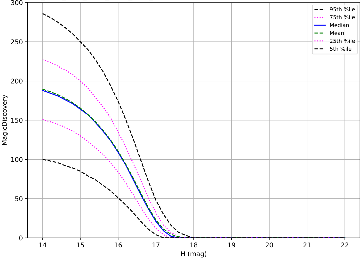
ddf_acor_sf25_lsf40_lsr20_v3.4_10yrs: Trojan 6 detections in 60 nights detection loss
