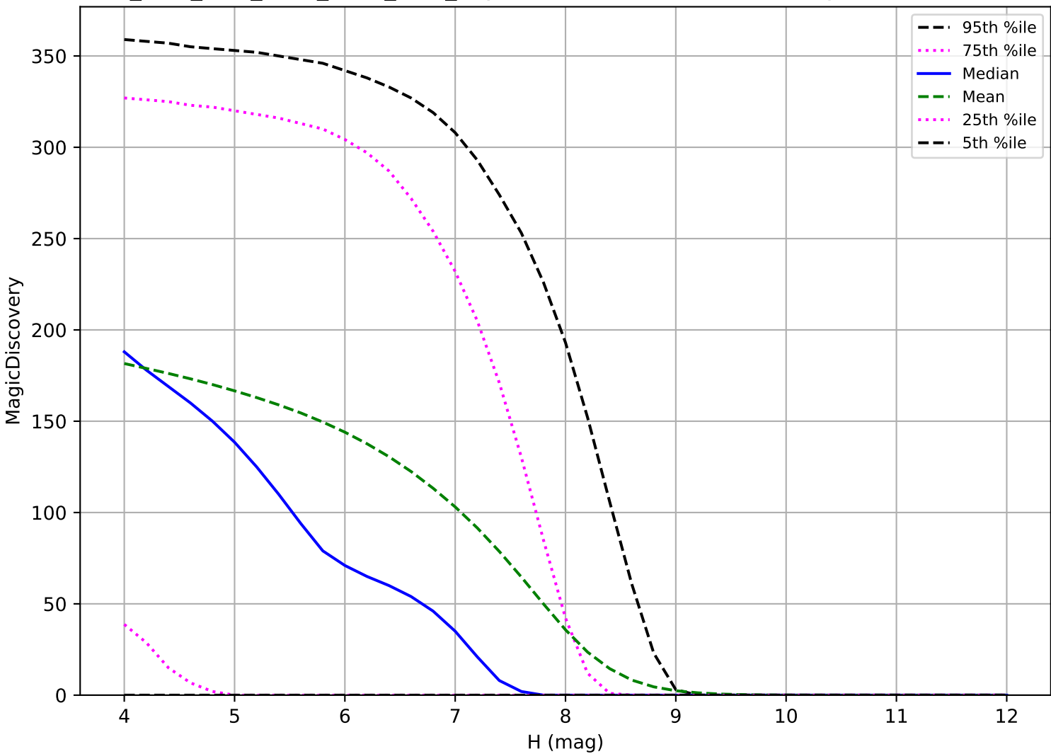
ddf_acor_sf25_lsf40_lsr20_v3.4_10yrs: TNO 6 detections in 60 nights detection loss
