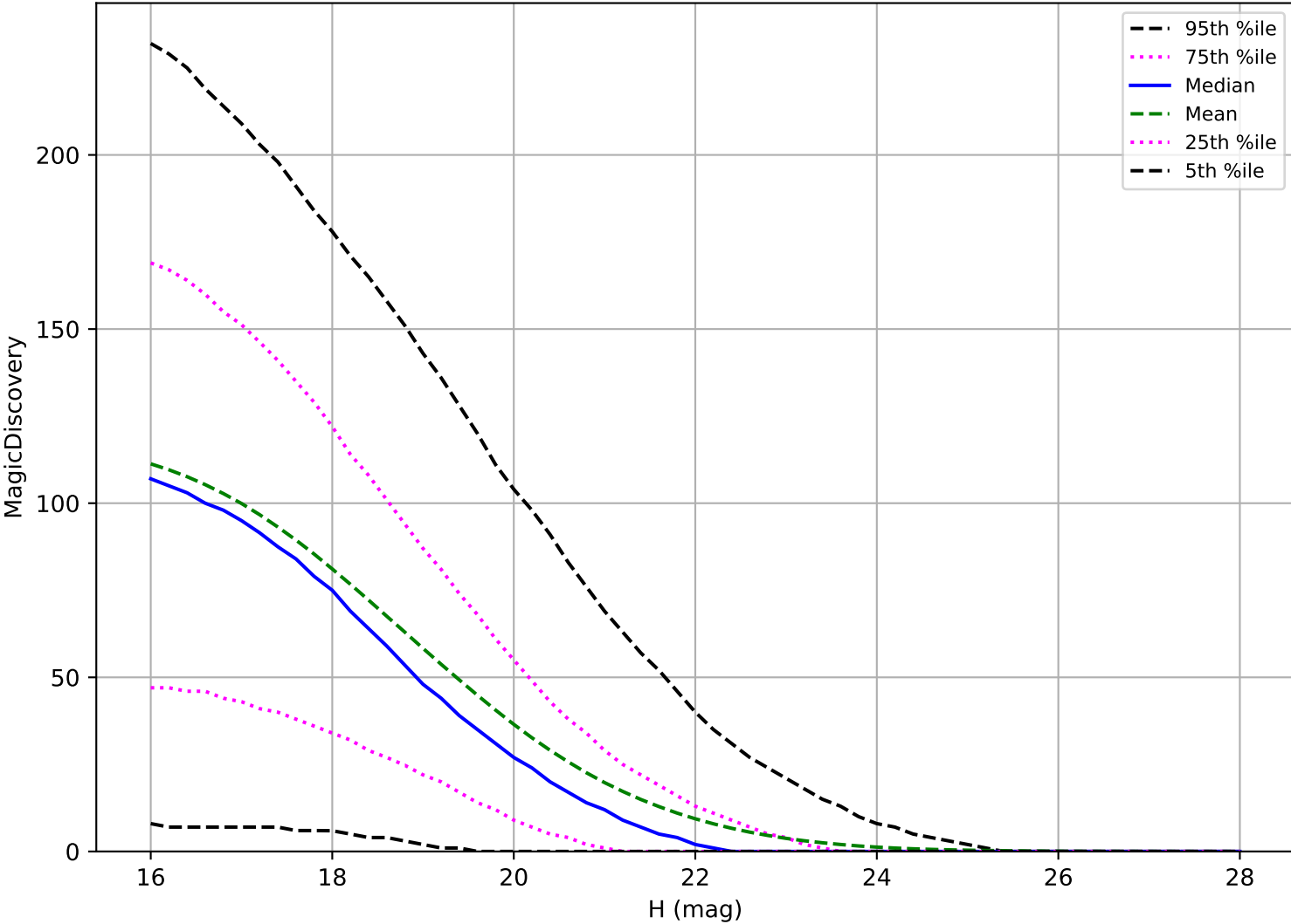
ddf_acor_sf25_lsf40_lsr20_v3.4_10yrs: PHA 6 detections in 60 nights detection loss
