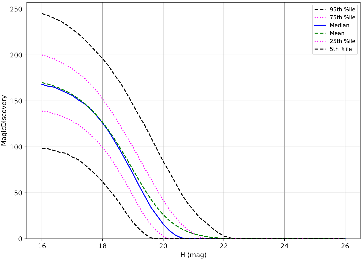
ddf_acor_sf25_lsf40_lsr20_v3.4_10yrs: MBA 6 detections in 60 nights detection loss
