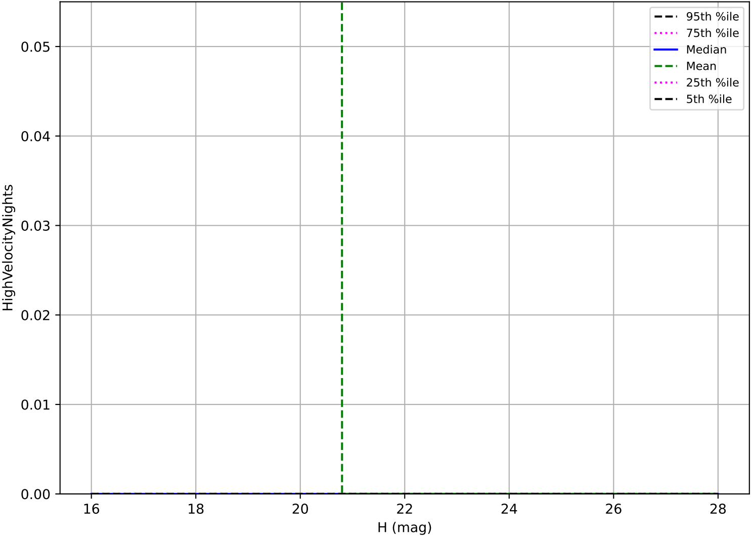
ddf_acor_sf25_lsf40_lsr20_v3.4_10yrs: Vatira High velocity pair detection loss
