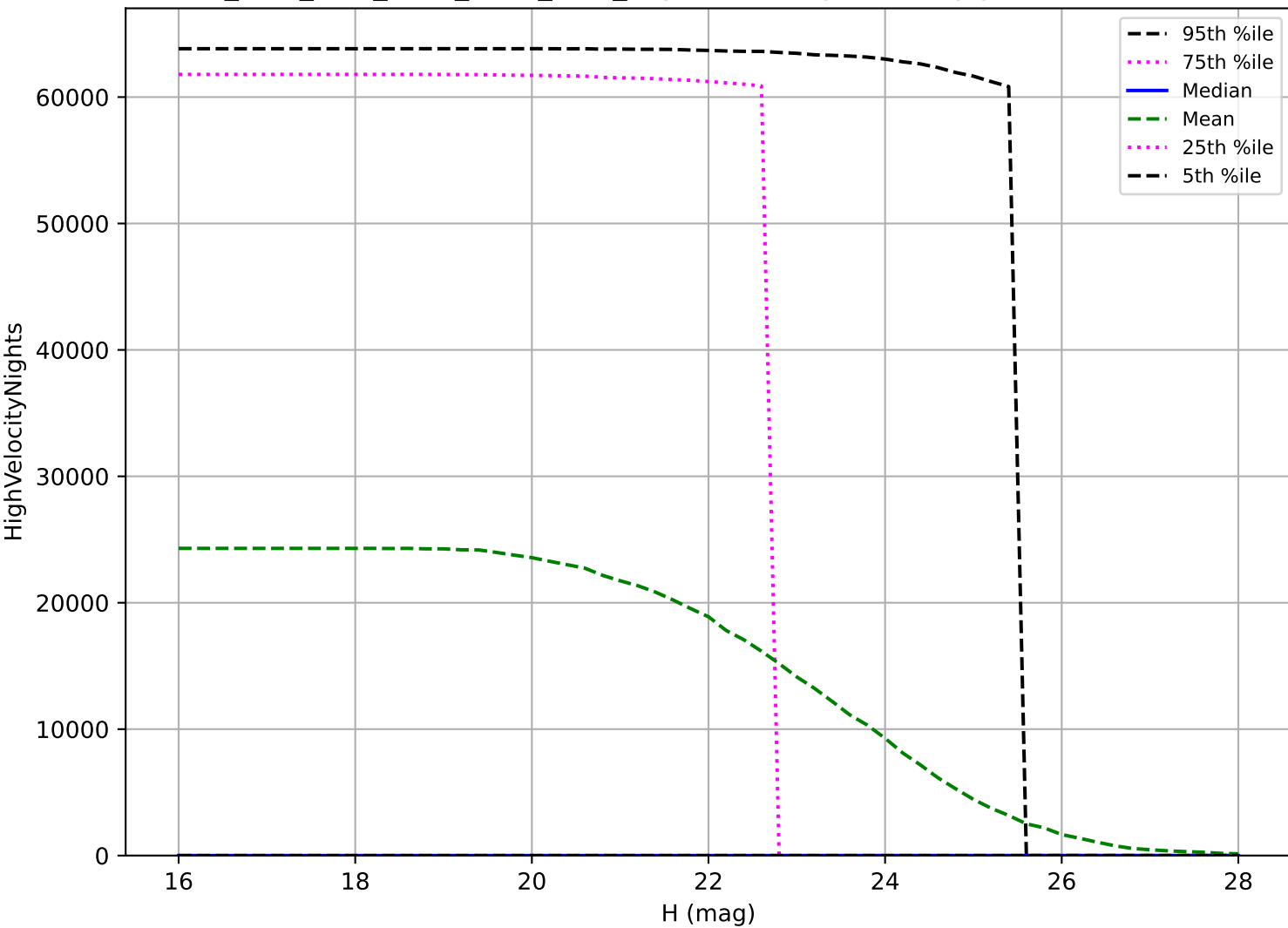
ddf_acor_sf25_lsf40_lsr20_v3.4_10yrs: PHA High velocity pair detection loss
