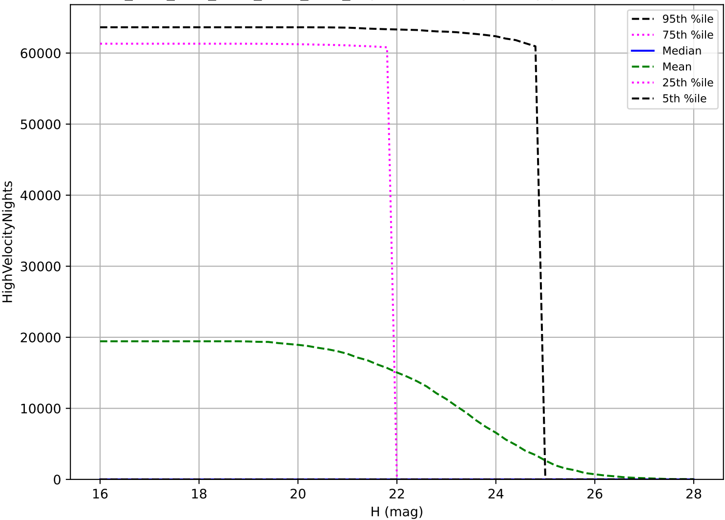
ddf_acor_sf25_lsf40_lsr20_v3.4_10yrs: NEO High velocity pair detection loss
