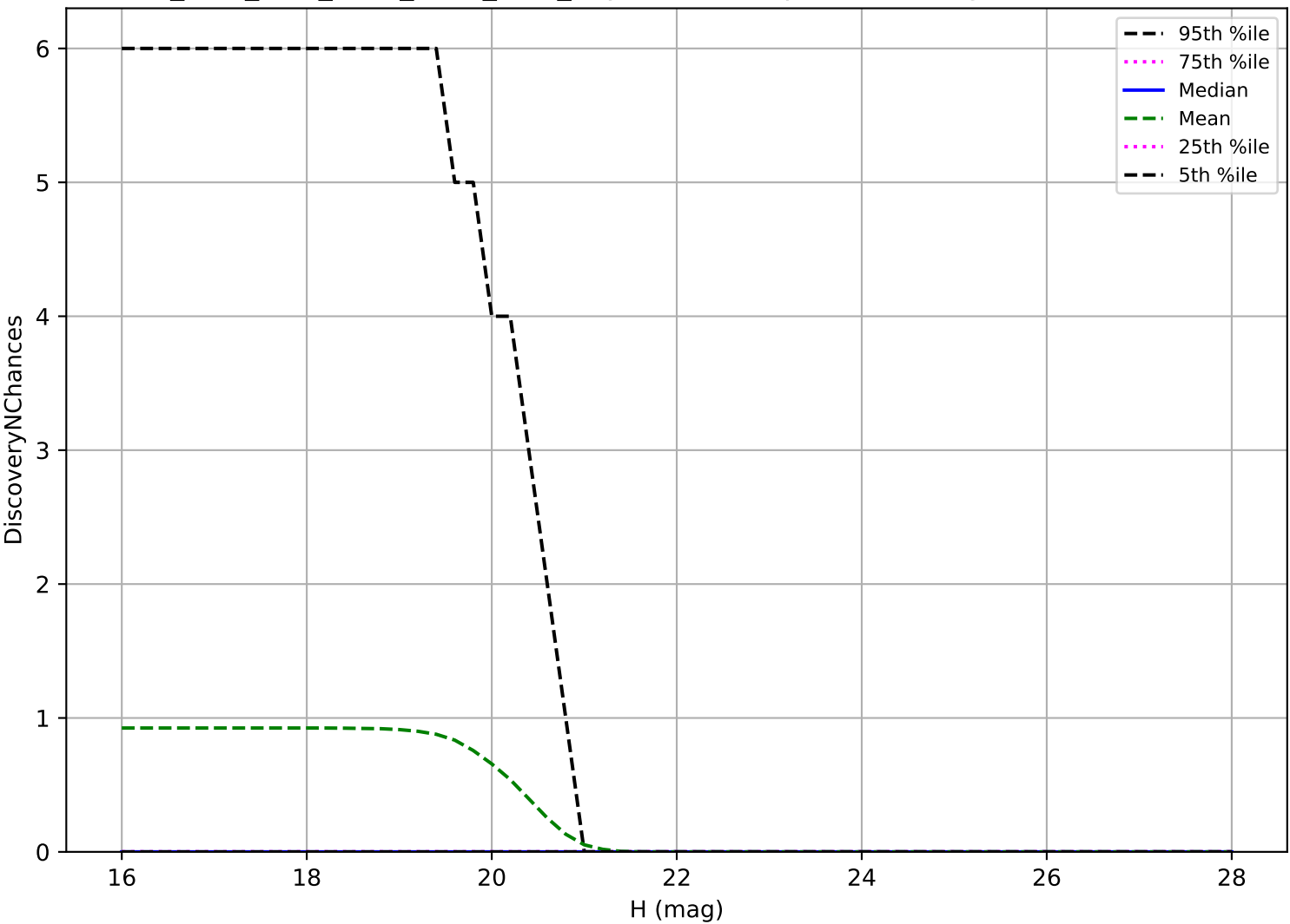
ddf_acor_sf25_lsf40_lsr20_v3.4_10yrs: Vatira 3 pairs in 15 nights detection loss
