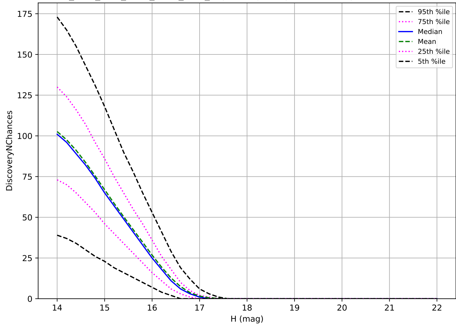
ddf_acor_sf25_lsf40_lsr20_v3.4_10yrs: Trojan 3 pairs in 15 nights detection loss
