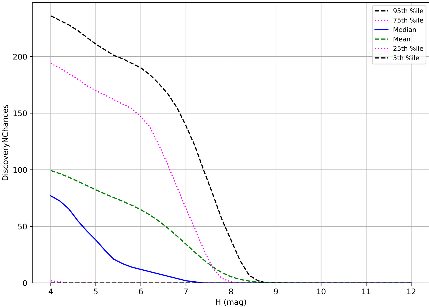
ddf_acor_sf25_lsf40_lsr20_v3.4_10yrs: TNO 3 pairs in 15 nights detection loss
