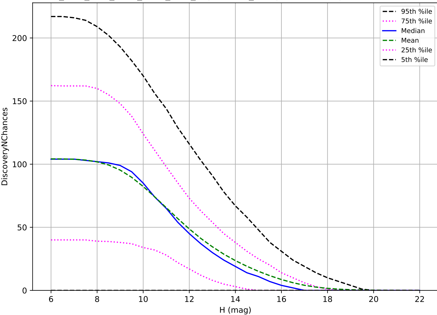
ddf_acor_sf25_lsf40_lsr20_v3.4_10yrs: OCC_r5 3 pairs in 15 nights detection loss
