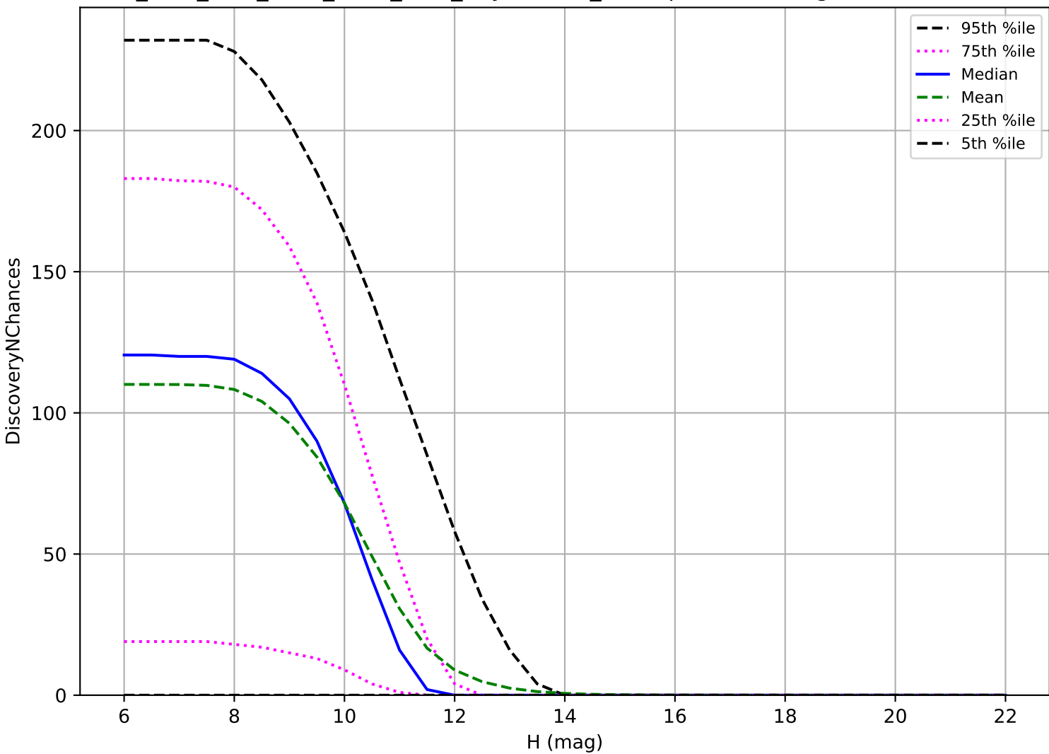
ddf_acor_sf25_lsf40_lsr20_v3.4_10yrs: OCC_r20 3 pairs in 15 nights detection loss
