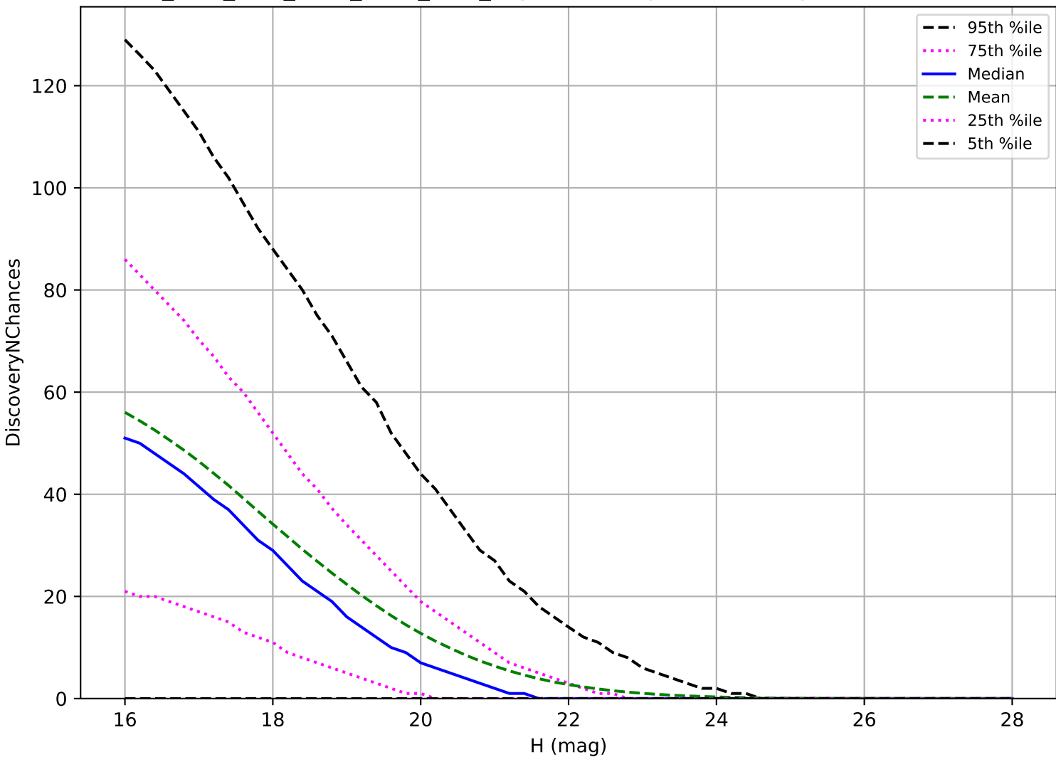
ddf_acor_sf25_lsf40_lsr20_v3.4_10yrs: NEO 3 pairs in 15 nights detection loss
