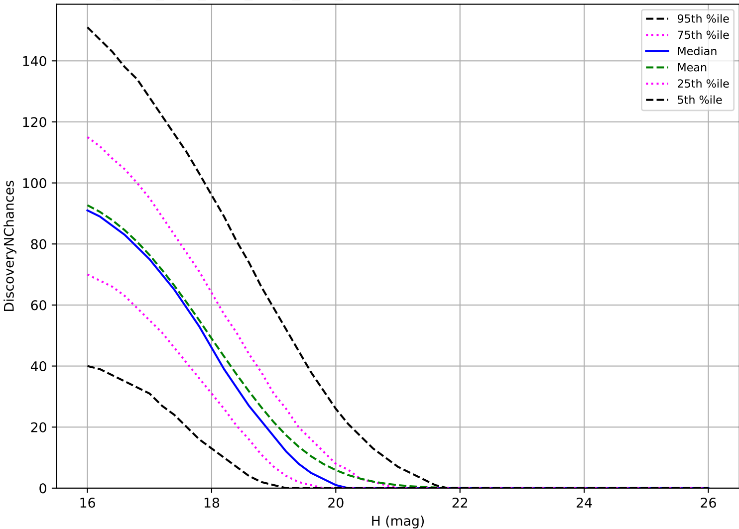
ddf_acor_sf25_lsf40_lsr20_v3.4_10yrs: MBA 3 pairs in 15 nights detection loss
