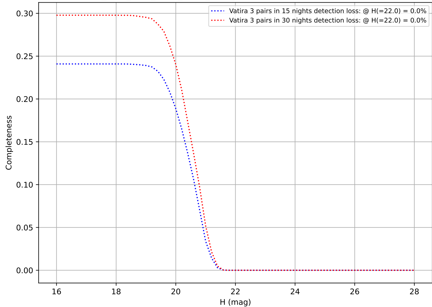
ddf_acor_sf25_lsf40_lsr20_v3.4_10yrs: DifferentialCompleteness
