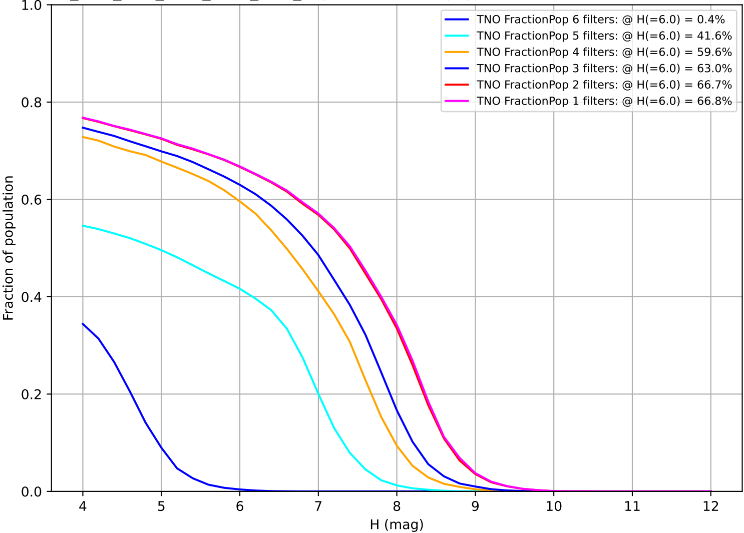
ddf_acor_sf25_lsf40_lsr20_v3.4_10yrs: Fraction of population with colors in X filters TNO
