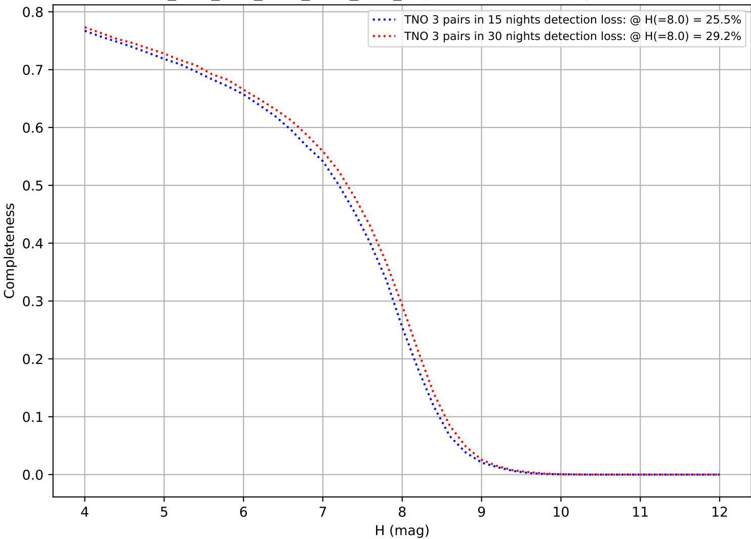
ddf_acor_sf25_lsf40_lsr20_v3.4_10yrs: DifferentialCompleteness
