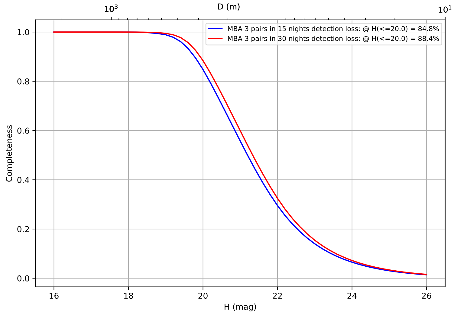
ddf_acor_sf25_lsf40_lsr20_v3.4_10yrs: CumulativeCompleteness
