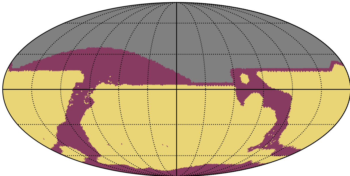
ddf_acor_sf25_lsf40_lsr20_v3.4_10yrs : RapidRevisits
