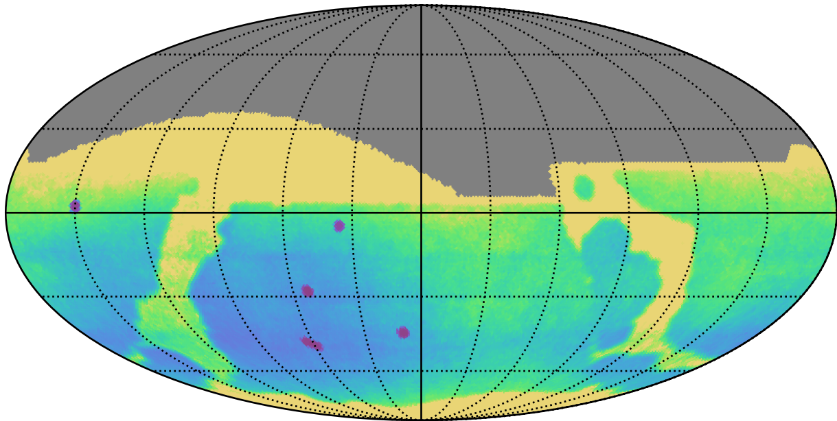
ddf_acor_sf25_lsf40_lsr20_v3.4_10yrs : Parallax Uncert @ 24.0
