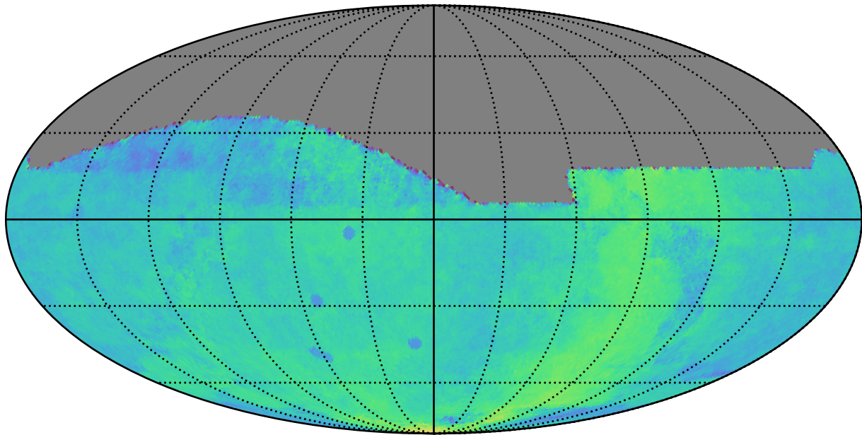
ddf_acor_sf25_lsf40_lsr20_v3.4_10yrs : Parallax Coverage @ 24.0
