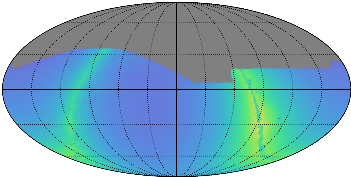
ddf_acor_sf25_lsf40_lsr20_v3.4_10yrs r: Nstars_no_crowding
