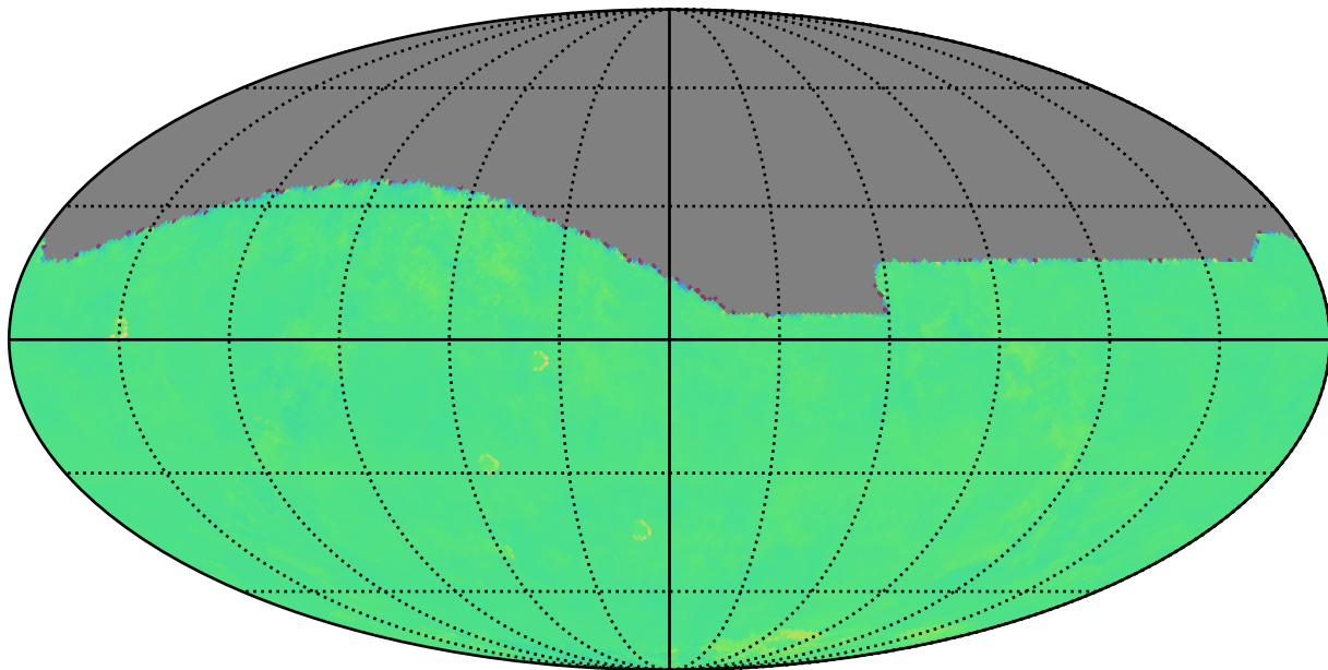
ddf_acor_sf25_lsf40_lsr20_v3.4_10yrs r: Kuiper rotTelPos
