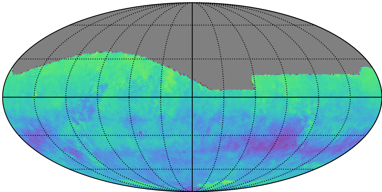
ddf_acor_sf25_lsf40_lsr20_v3.4_10yrs r: Kuiper rotSkyPos
