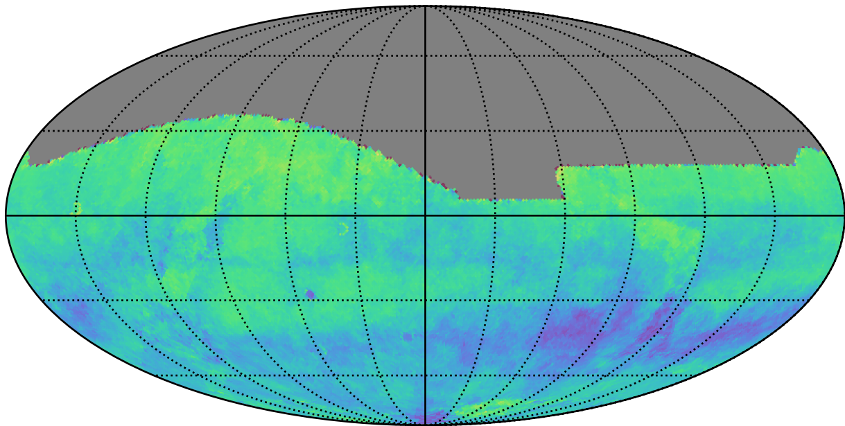
ddf_acor_sf25_lsf40_lsr20_v3.4_10yrs i: Kuiper rotSkyPos
