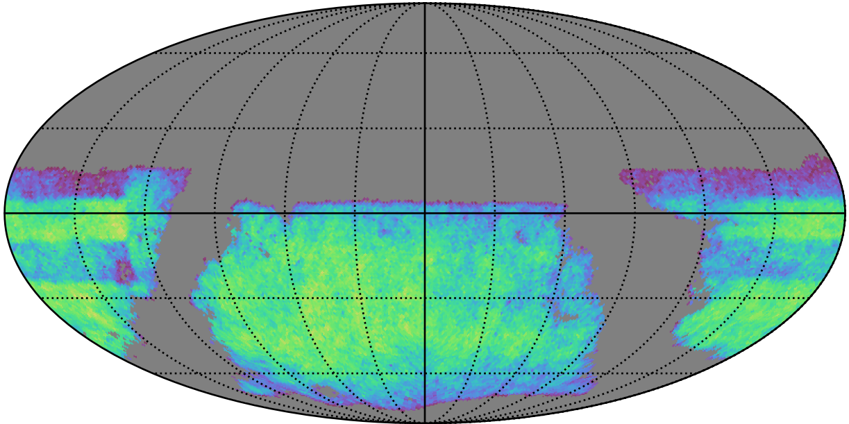
ddf_acor_sf25_lsf40_lsr20_v3.4_10yrs i band non-DD year 2: ExgalM5WithCuts
