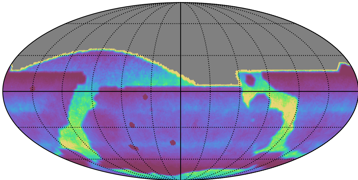
ddf_acor_sf25_lsf40_lsr20_v3.4_10yrs : DCRprecision
