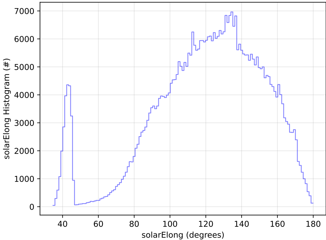
ddf_acor_sf25_lsf40_lsr20_v3.4_10yrs WFD z band: solarElong Histogram
