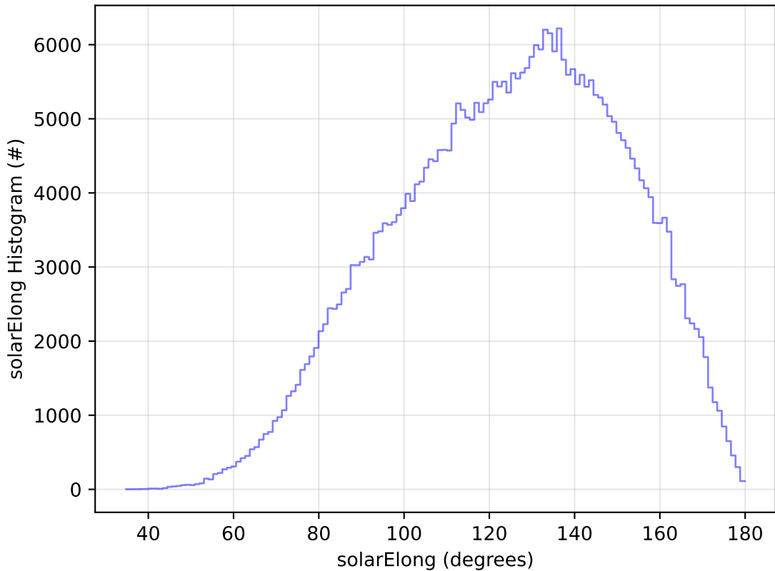
ddf_acor_sf25_lsf40_lsr20_v3.4_10yrs WFD y band: solarElong Histogram
