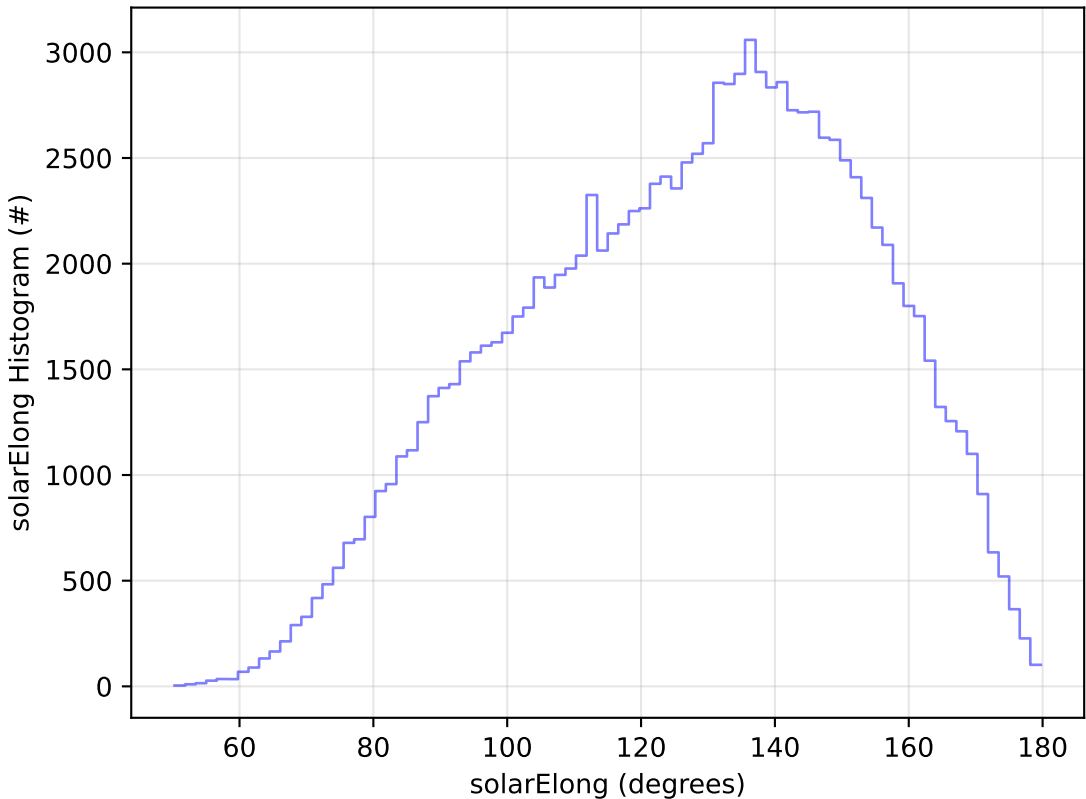
ddf_acor_sf25_ls40_lsr20_v3.4_10yrs WFD u band: solarElong Histogram
