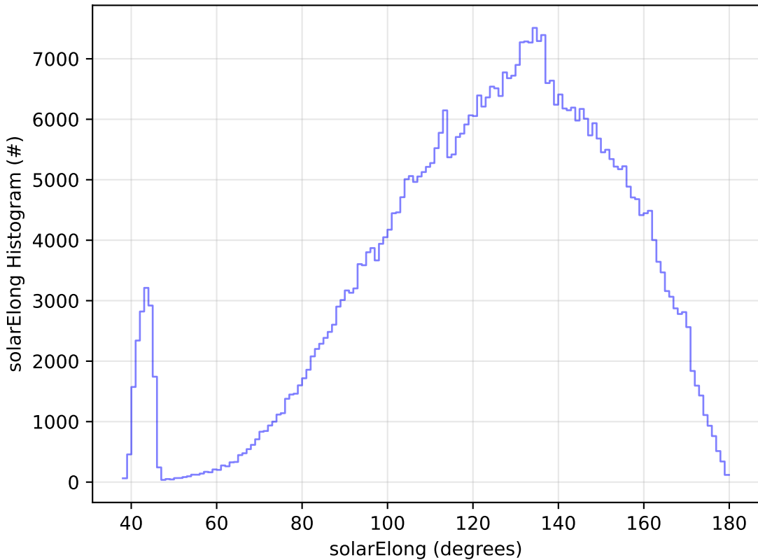
ddf_acor_sf25_lsf40_lsr20_v3.4_10yrs WFD r band: solarElong Histogram
