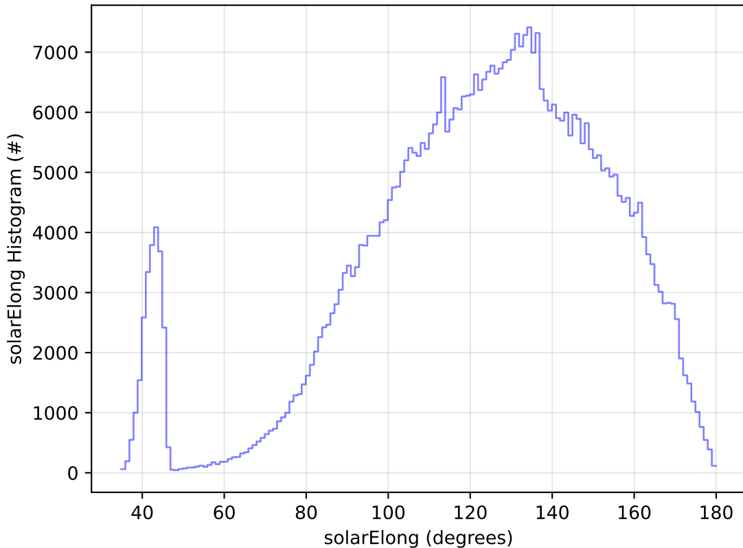
ddf_acor_sf25_lsf40_lsr20_v3.4_10yrs WFD i band: solarElong Histogram
