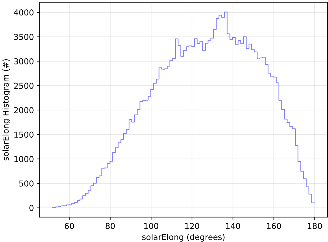
ddf_acor_sf25_lsf40_lsr20_v3.4_10yrs WFD g band: solarElong Histogram
